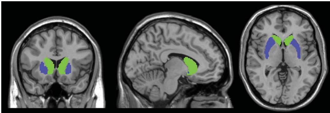
Fig. 1. The bilateral striatum areas were selected as ROIs based on AAL atlas. The bilateral putamen was labeled with blue, and caudate were labeled with green. ROI, region of interests; AAL, Automated Anatomical Labeling.
