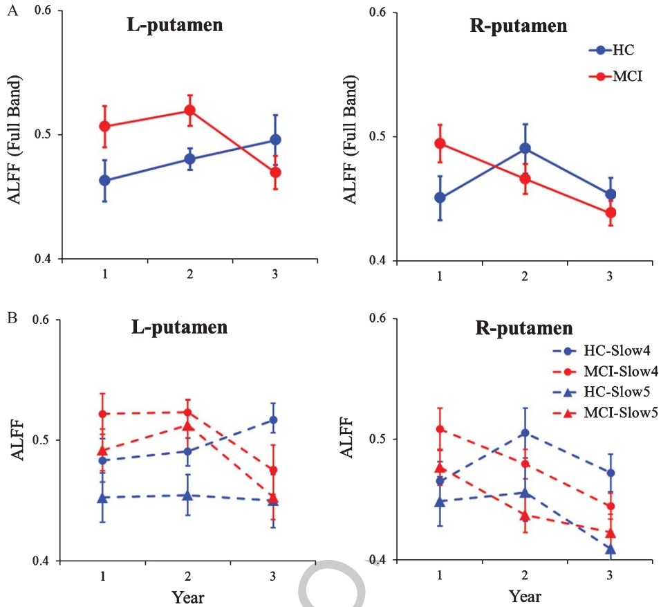
Fig. 2. Longitudinal trajectories of ALFF [full band (A), slow-4 band and slow-5 band (B)] in the bilateral putamen of MCI and HC groups. ALFF, amplitude of low frequency fluctuations; HC, healthy control; MCI, mild cognitive impairment; L, left; R, right.
