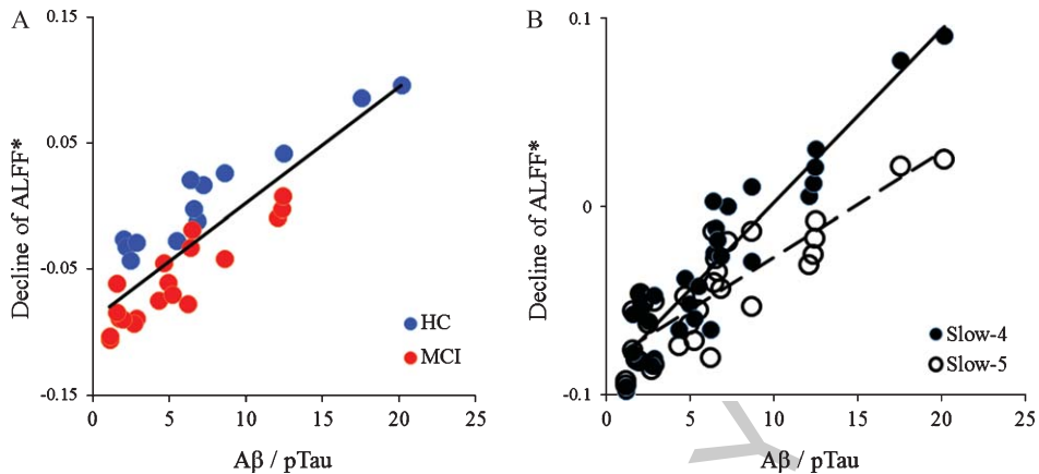
Fig. 3. Associations between baseline Aβ/pTau ratio and decline of ALFF values in the R-putamen. A) The association between Aβ/pTau ratio and decline of ALFF in R-putamen across HC and MCI groups. B) The association between Aβ/pTau ratio and decline of ALFF between slow-4 and slow-5 bands. *All models were adjusted for age and group (MCI versus HC). Note. Decline of ALFF was computed as the baseline and two-year follow-up difference with lower value indicating greater decline; lower value of Aβ/pTau ratio indicates worse AD pathology. ALFF, amplitude of low frequency fluctuations; HC, healthy control; MCI, mild cognitive impairment.
