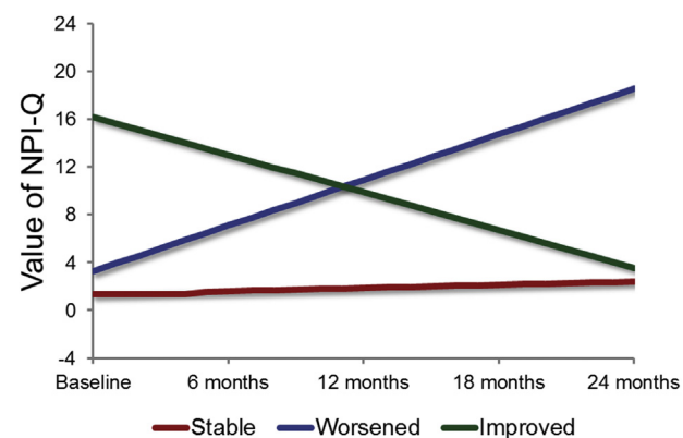
FIGURE 1. Graphical representation of NPI-Q scores over time by the latent class. Higher scores of NPI-Q indicated worse NPS.
