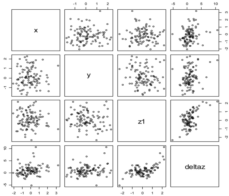
Figure 2. Example of simulated data when \sigma = 1 where the distributions of x , y , z_1 are standard normal (the upper left 3 by 3 plots) and the relationships between z to x (as linear), to y (as linear) and to z_1 (as cubic).
