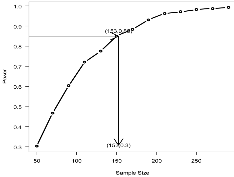
Figure 4. Power curve for Chen et al (2010). The estimated sample size for power of 0.85 is 153
