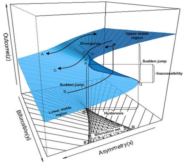
Figure 1. Cusp catastrophe model for outcome measures ( Z ) in the equilibrium plane with asymmetry control variable ( X ) and bifurcation control variable ( Y ). (Annotated by the authors with the original graph produced by Grasman's R package "cusp")
